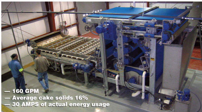
2 meter 3DP Belt Press, Reservoir – Alum Water Treatment Plant.
